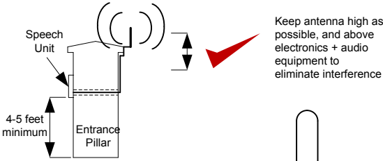
Fig.1. Side View
